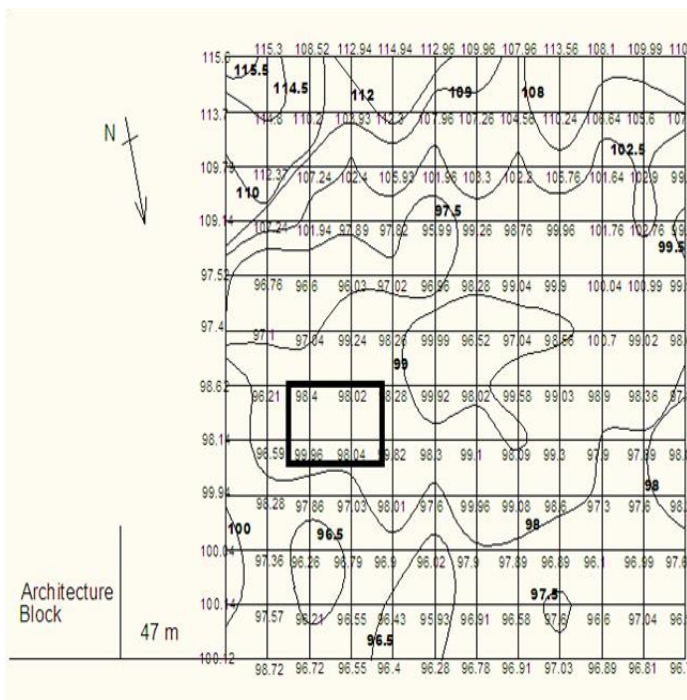
Fig. 5: Contour Plan
