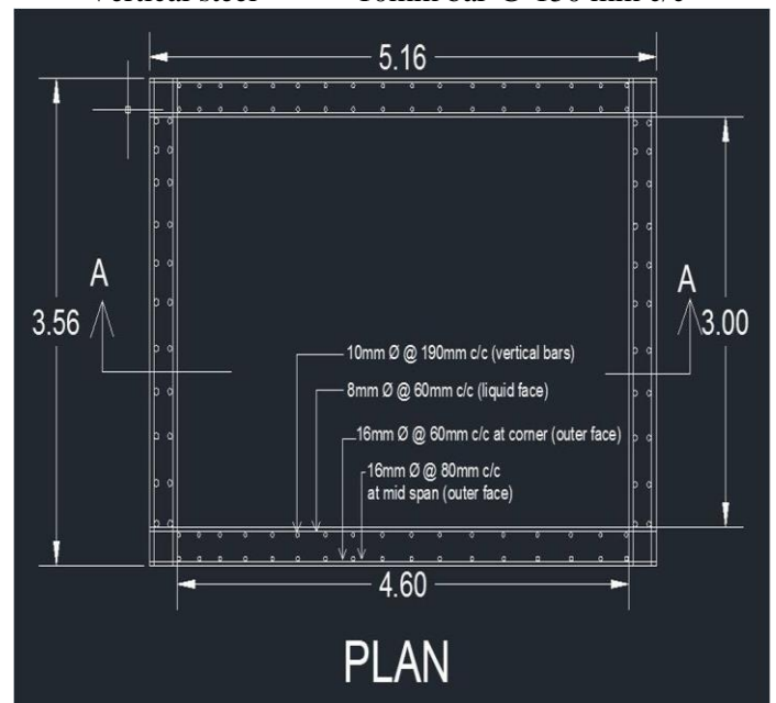
Fig. 6: Reinforcement Details
