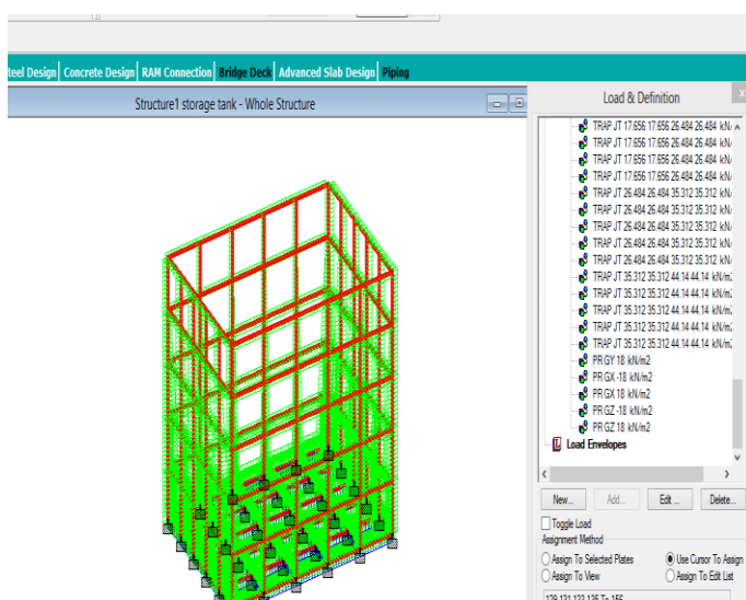
Fig. 8: Loading details of Storage tank
