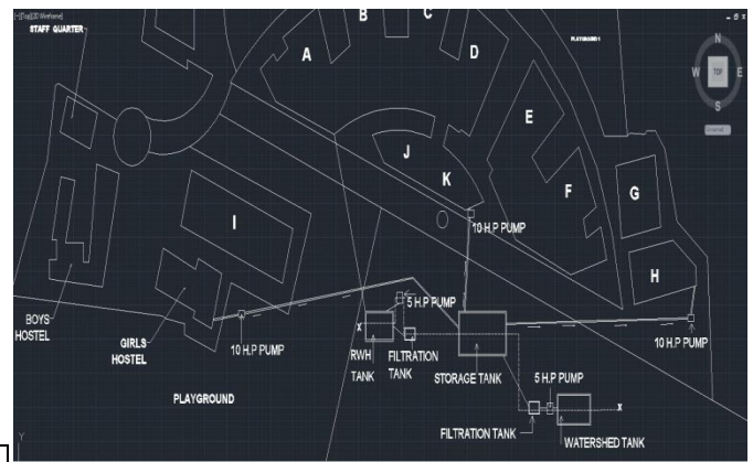
Fig. 12: Distribution Layout
