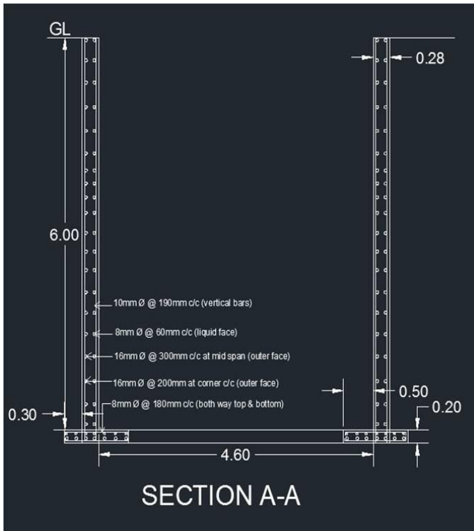
Fig. 7: Section of watershed tank (watershed)
