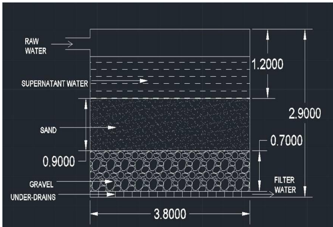
Fig. 10: Slow Sand Filter
