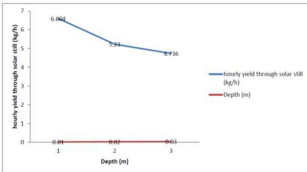
Figure 16: Variation of yield with water depth
