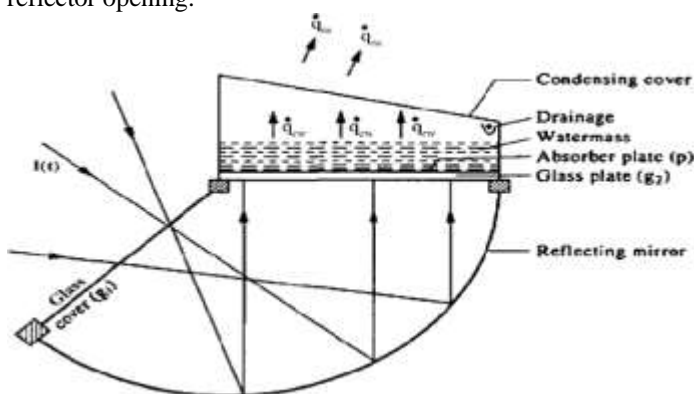
Figure 3: Inverted Solar Still
