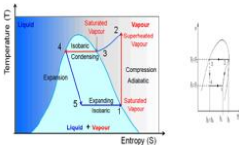
Fig. 1.3 P-h diagram of VCRS system
