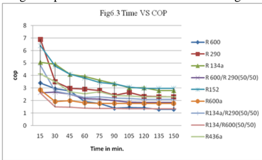
Fig 1.10 Time VS COP
