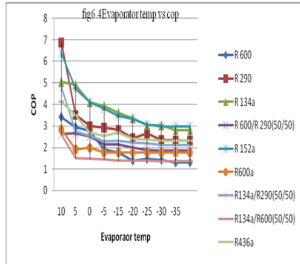
Fig.1.11 Evaporator temperature vs cop
