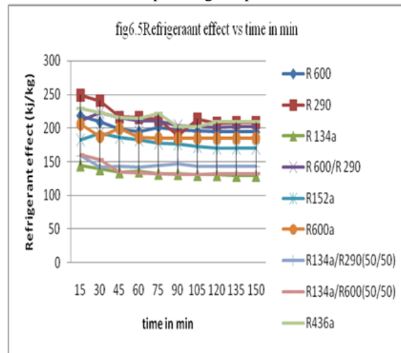
Fig 1.12 Refrigerant effect vs time in min
