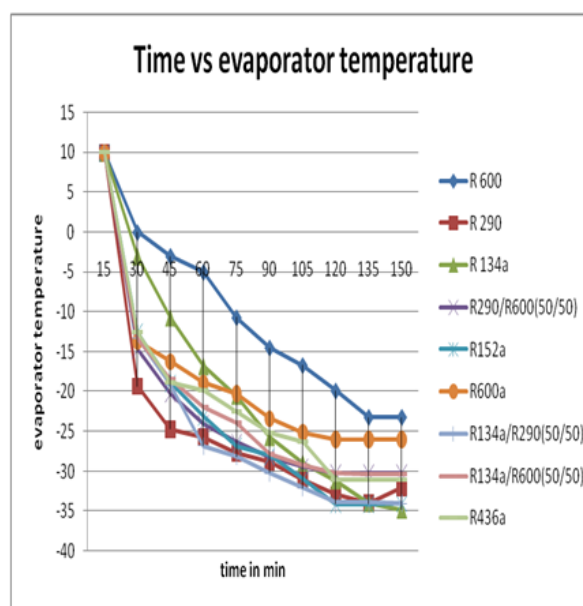
Fig 1.8 Time VS evaporator temperature
