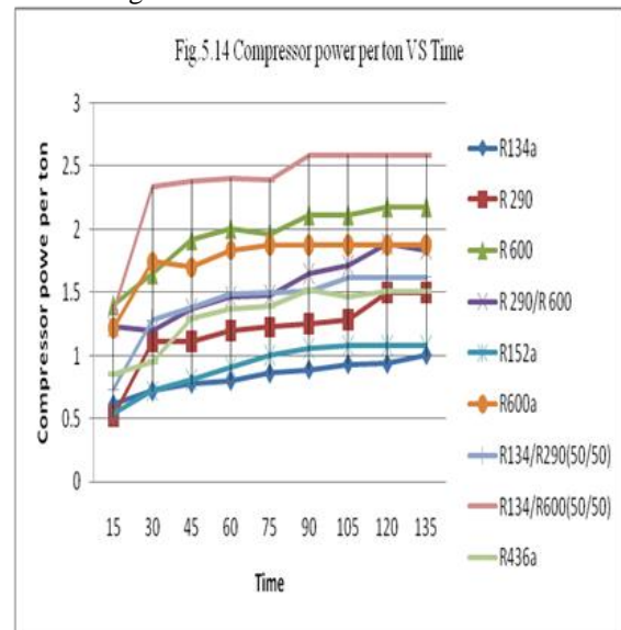
Fig 1.20 Compressor power per ton vs time
