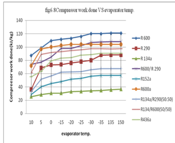
Fig 1.15 Compressor work done vs Evaporator temp
