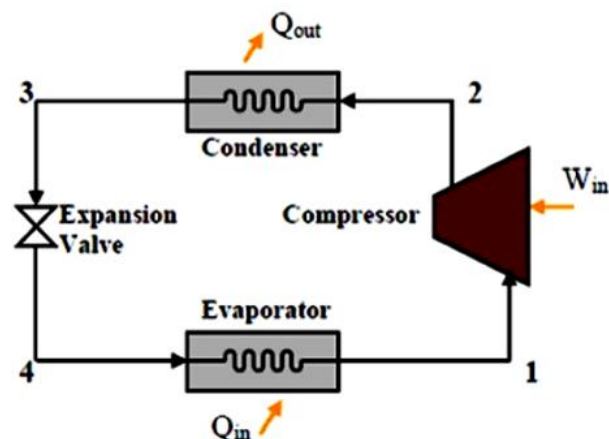
Fig. 1.1 VCRS system
