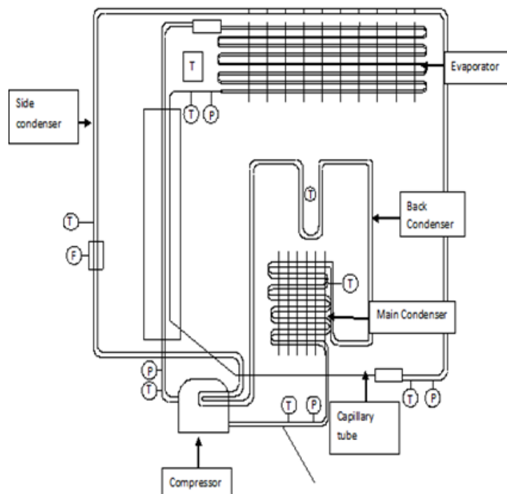
Fig.1.6 Line diagram of experiment
