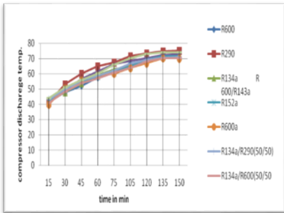
Fig. 1.9 Time VS discharge temp.
