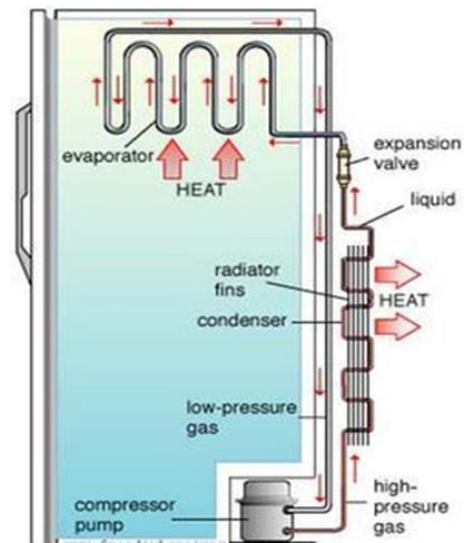
Fig. 1.4 Domestic Refrigerator
