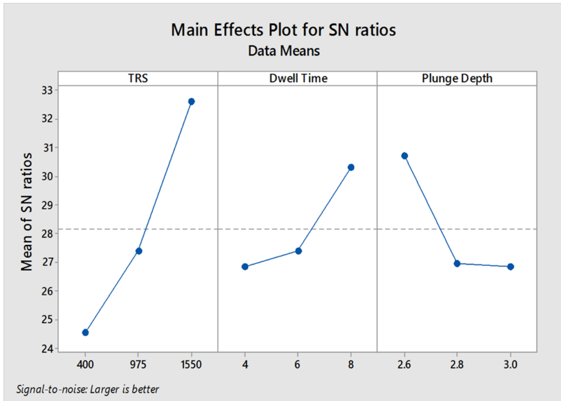
Fig. 5.1 Effect of process parameters for S/N ratio (tensile strength)
