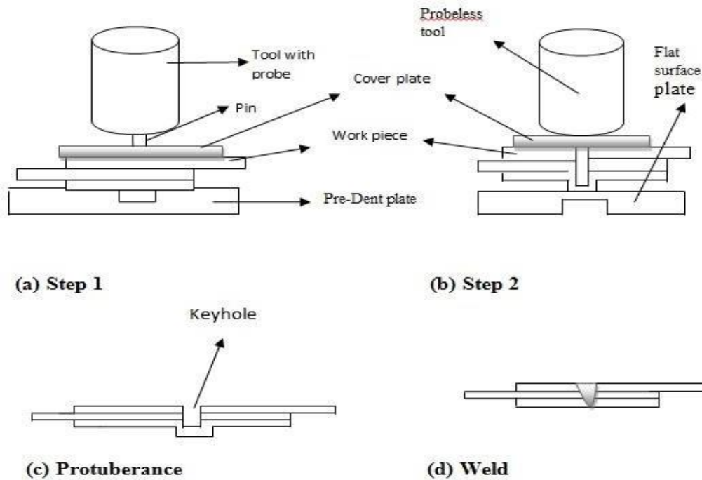
Fig 3.4 Experimental Tool and workpiece arrangement
