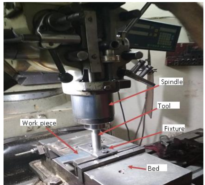
Fig.3.5 Flat Friction Stir Spot Welding Setup
