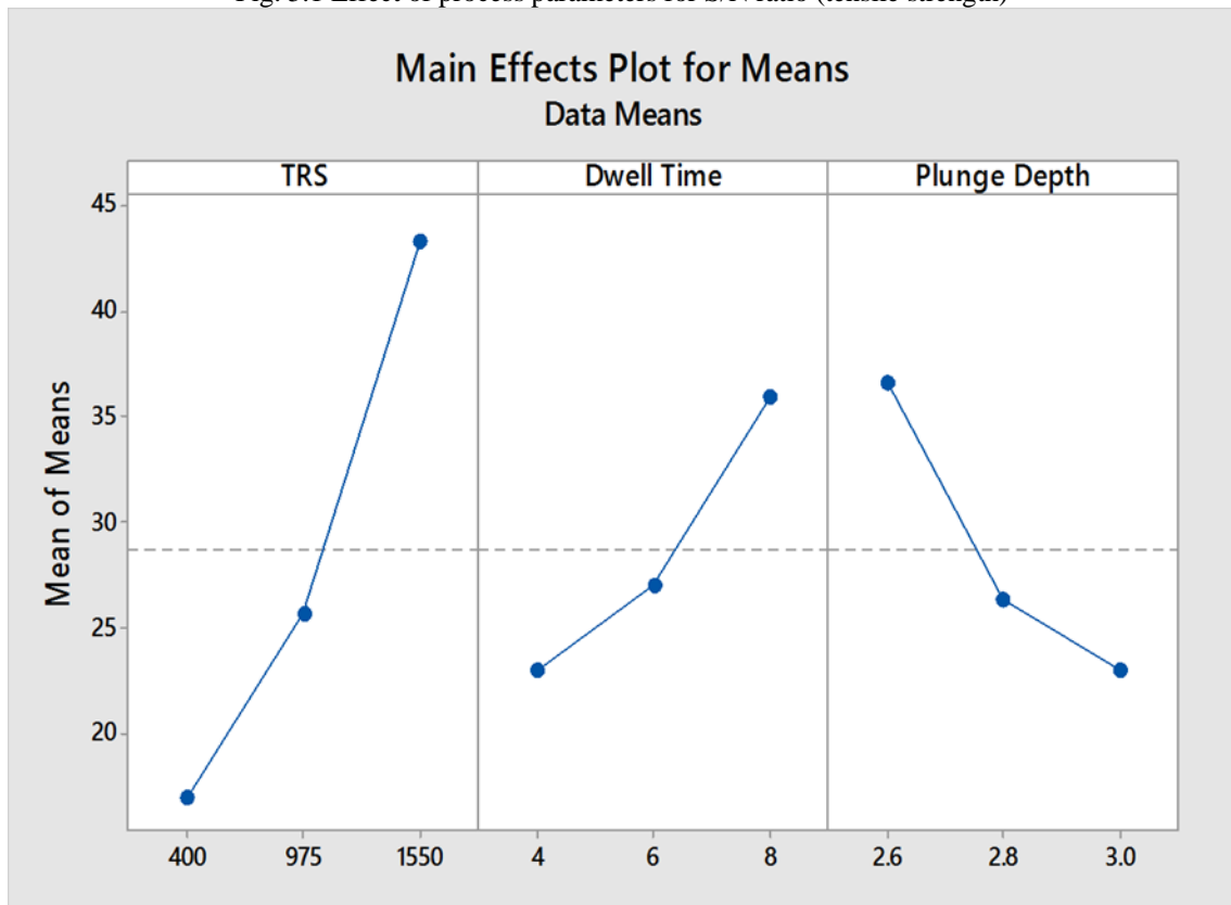
Fig. 5.2 Effect of process parameters for Mean (tensile strength)
