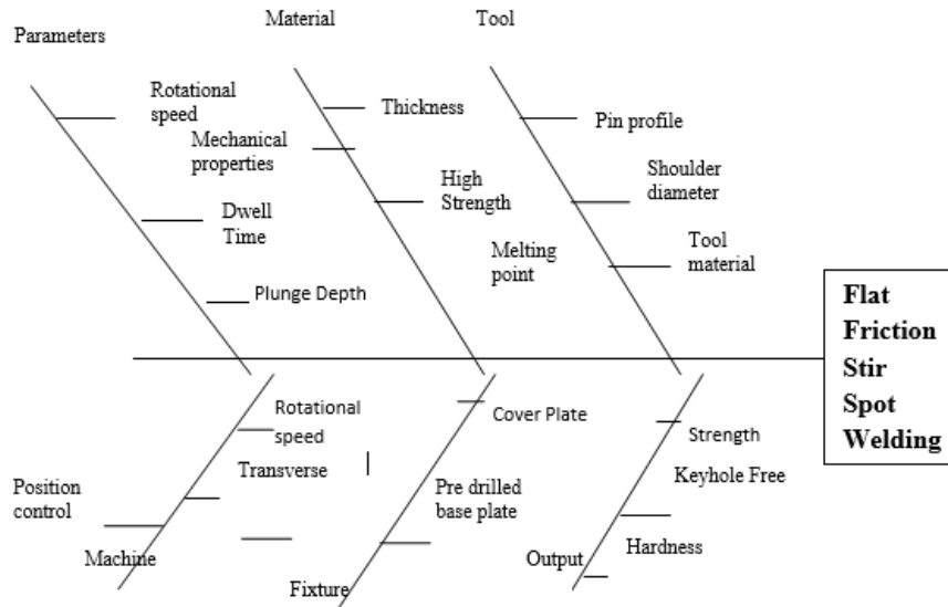
Fig.3.3 Ishikawa diagram of Flat-FSSW process
