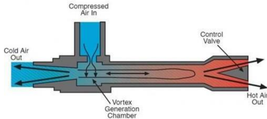
Fig 1.2 Ranque -Hilsch vortex tube
