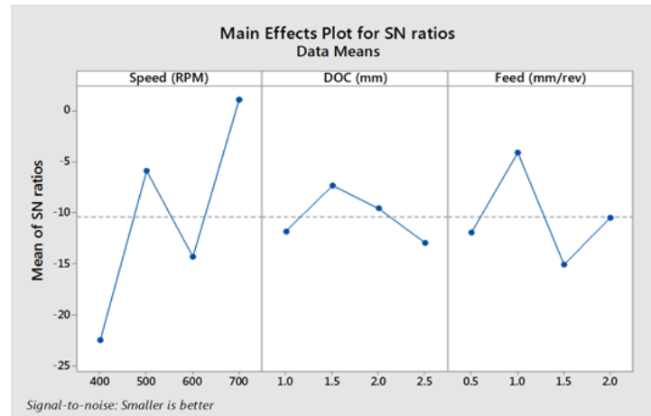
Fig 5.1: Main Effects Plot for S/N Ratios
