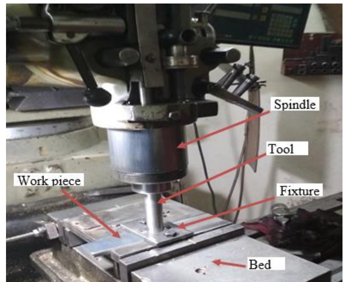
Fig.3.5 Flat Friction Stir Spot Welding Setup
