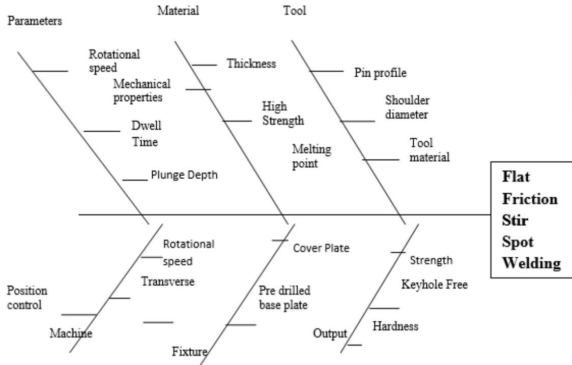
Fig.3.3 Ishikawa diagram of Flat-FSSW process
