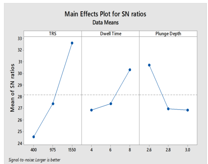
Fig. 5.1 Effect of process parameters for S/N ratio (tensile strength)
