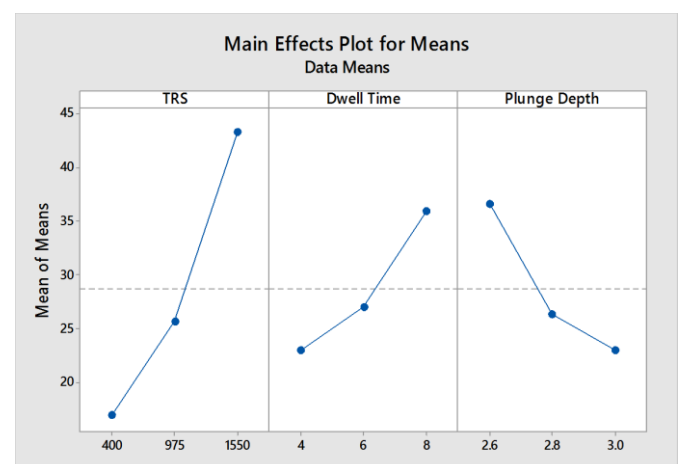
Fig. 5.2 Effect of process parameters for Mean (tensile strength)
