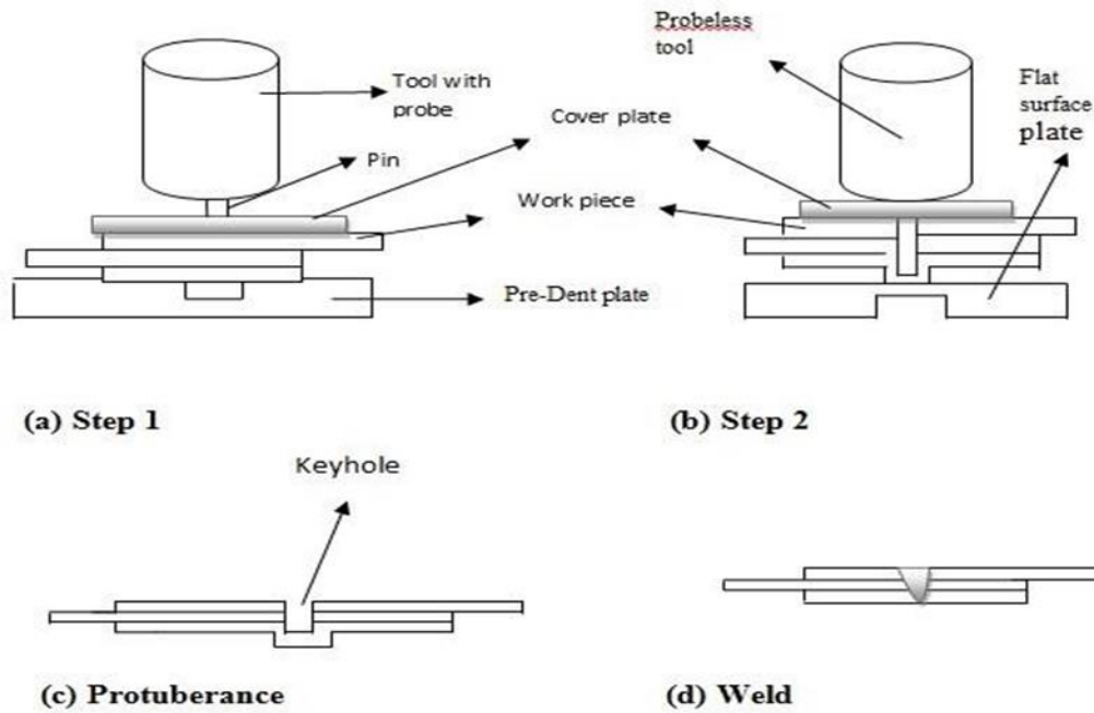
Fig 3.4 Experimental Tool and workpiece arrangement
