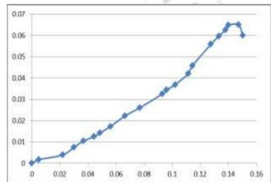
Fig-3.3: Stress strain curve of tensile test
