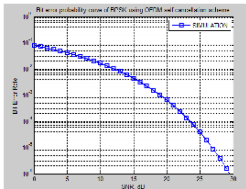
Fig 5:- Best BER performance with ICI cancellation at zero phase noise variance
