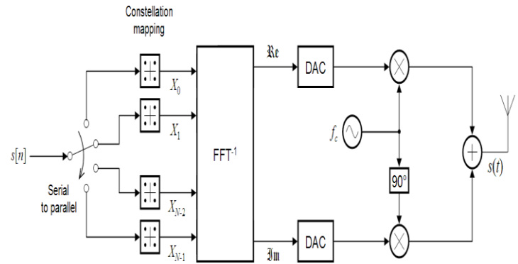
Fig 3 TRANSMITTER
