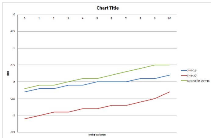
Fig 6: BER at different phase noise variance at SNR=15db and 20db
