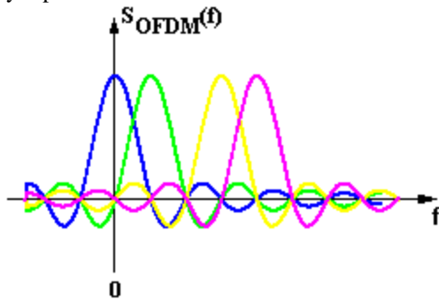
Fig.2:-An example of OFDM with 4 different signal shown in different colour
