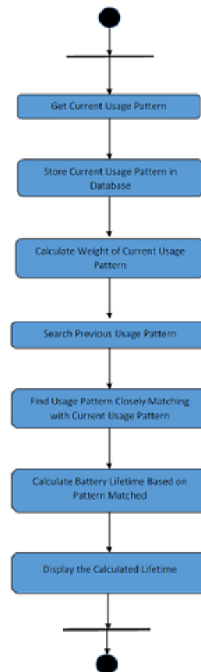
Figure 3. Activity Diagram
