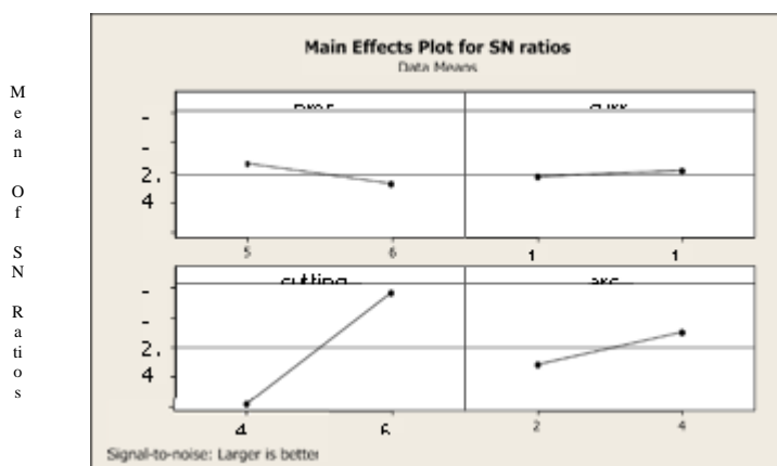
Graph 5.1 Effects of various factors on S / N Ratio of MRR
