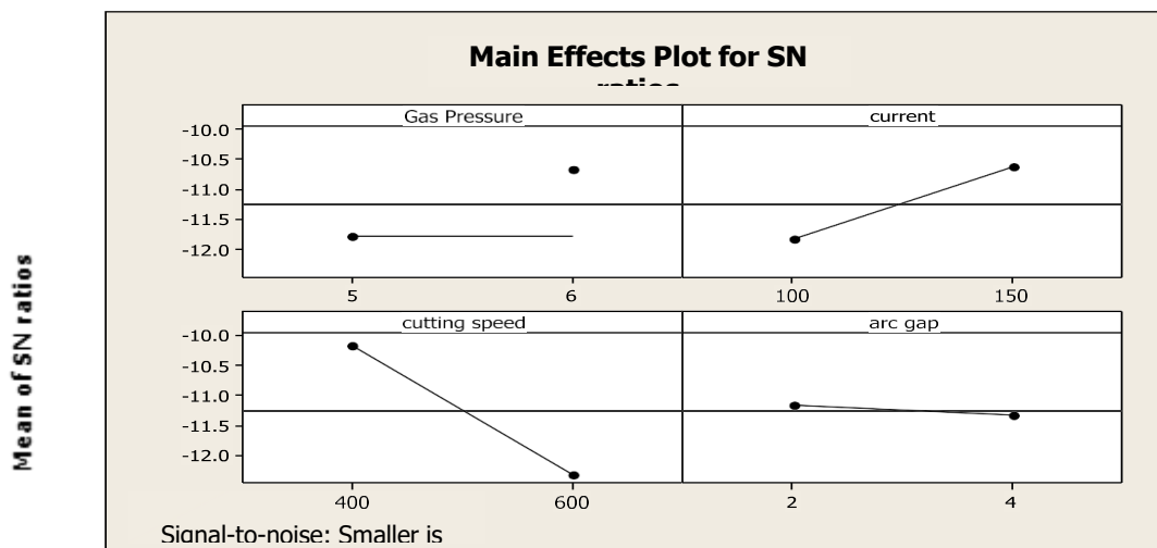
Graph 5.3 Effects of various factors on S / N Ratio of SR
